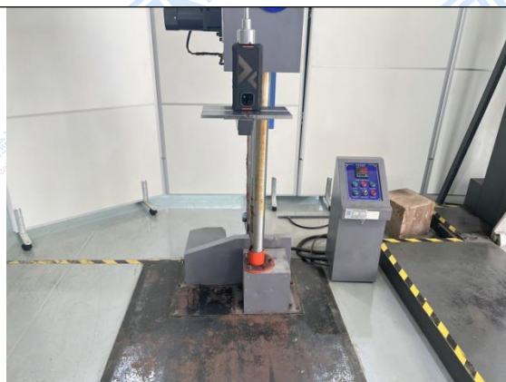
Fig.56 Test setup- Face (4)
