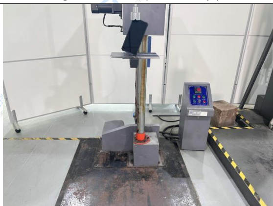
Fig.65 Test setup- Corner (7)
