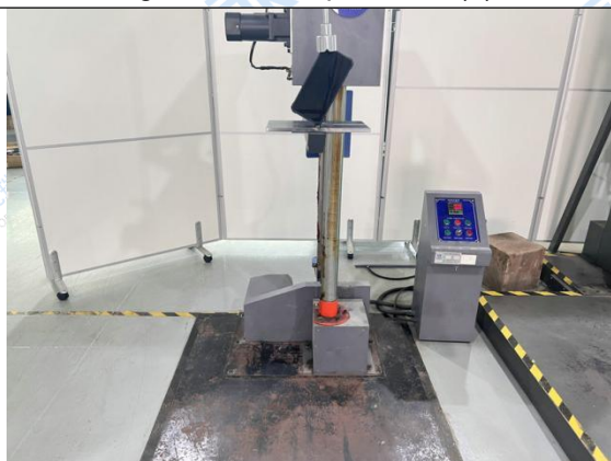
Fig.61 Test setup- Corner (3)
